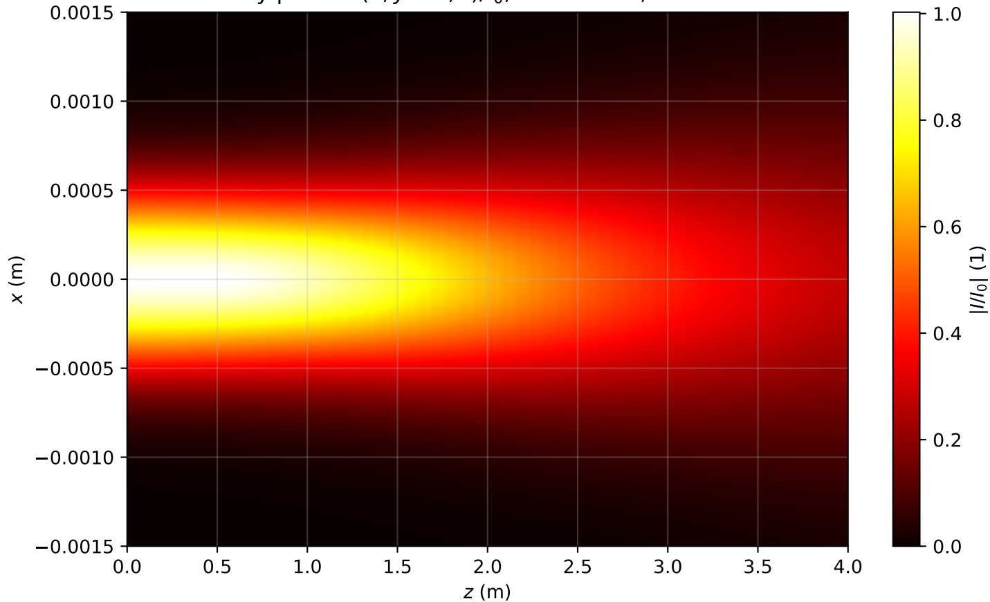
Intensity profile I(x, y = 0, z)/I_0 , \text{Pin}=0.3\text{Pcr} , artificial time
